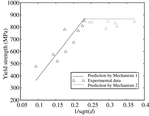
Fig. 3. The yield strength of nanocrystalline Cu versus the grain size 1/\sqrt{d} (nm)^{-1/2}
