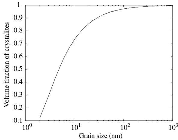
Fig. 1. The volume fraction of crystallites as a function of grain size
