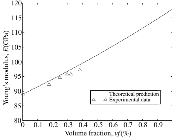
Fig. 2. The effective Young's modulus of bulk Zr_{53}Ti_5Ni_{10}Cu_{20}Al_{12} alloy versus the volume fraction of crystallites
