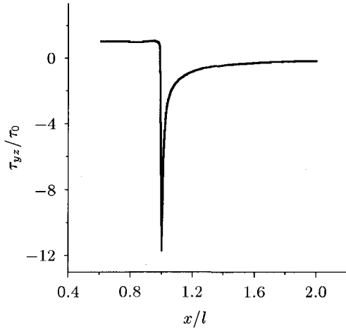
Fig.6 The stress along the crack line versus x/l for a/2\beta l = 0.001
