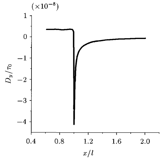
Fig.7 The electric displacement along the crack line versus x/l for a/2\beta l = 0.001
