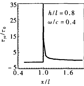
Fig.3 The variation of the stress along the crack line for a/(2\beta l) = 0.0005 .
